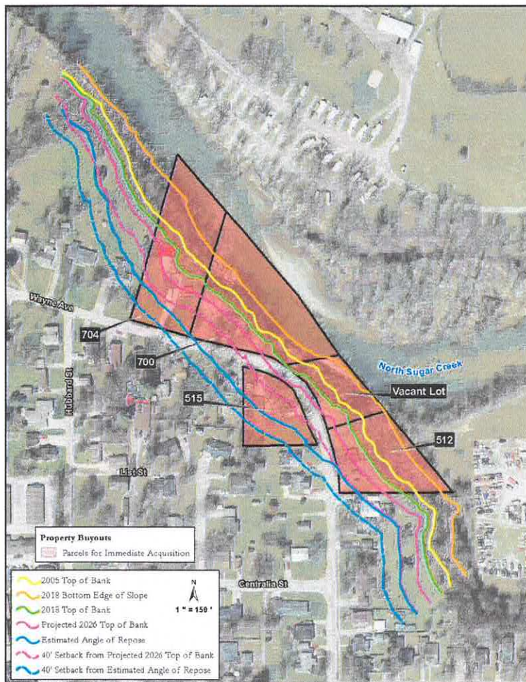
Figure 25 Historical and Predicted Sugar Creek Movement
