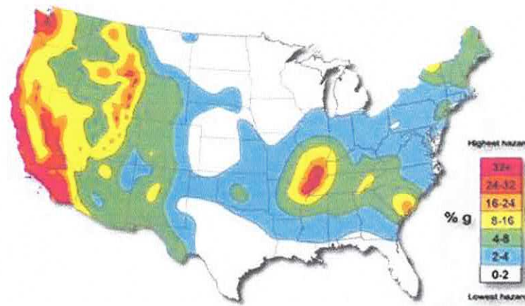
Figure 9 Earthquake Hazard Areas in the US
