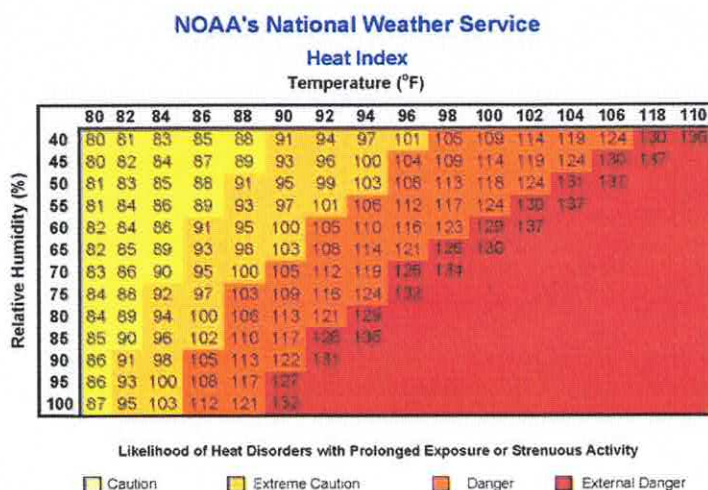
Figure 12 Heat Index Chart
