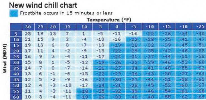
Figure 13 NWS Wind Chill Chart
