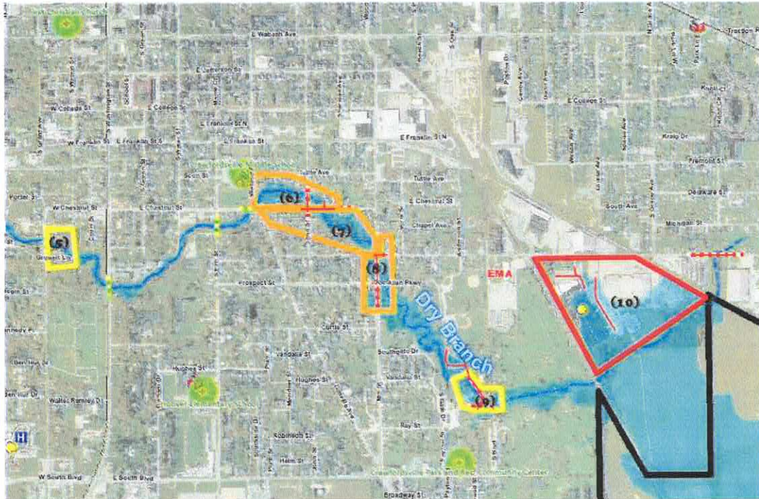
Figure 18 Potential Flood Impact Areas, Crawfordsville, IN
